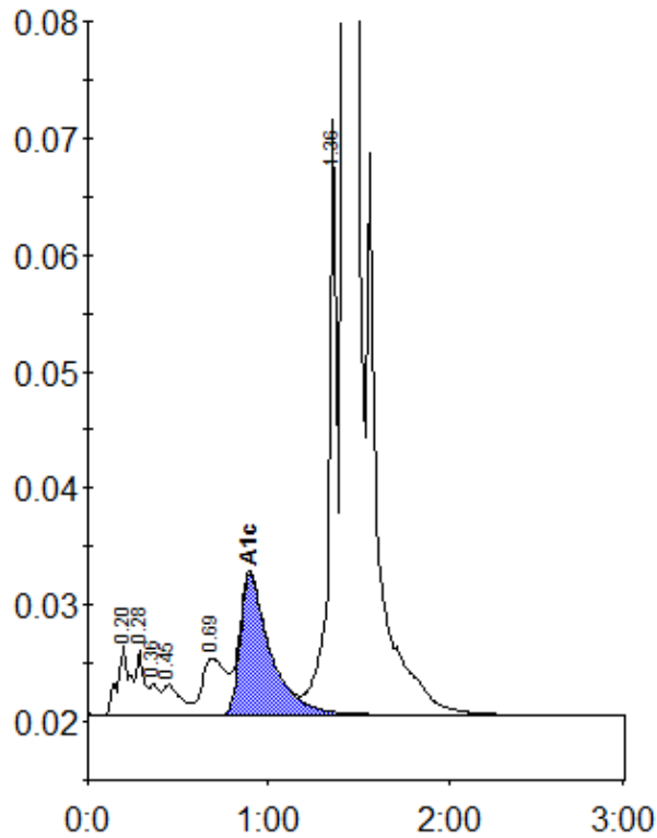
Peak table - ID: 10530247
